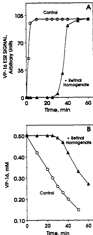
FIGURE 4: Time course of VP-16 phenoxyl radicals (A) as measured by ESR and of VP-16 oxidation (B) the measured by HPLC during tyrosinase-catalyzed VP-16 oxidation in the presence or absence of retinal homogenates. Incubation conditions: Retinal homogenate contained 7.0 mg of protein/mL. Other conditions were as given in the legend of Figure 3.
